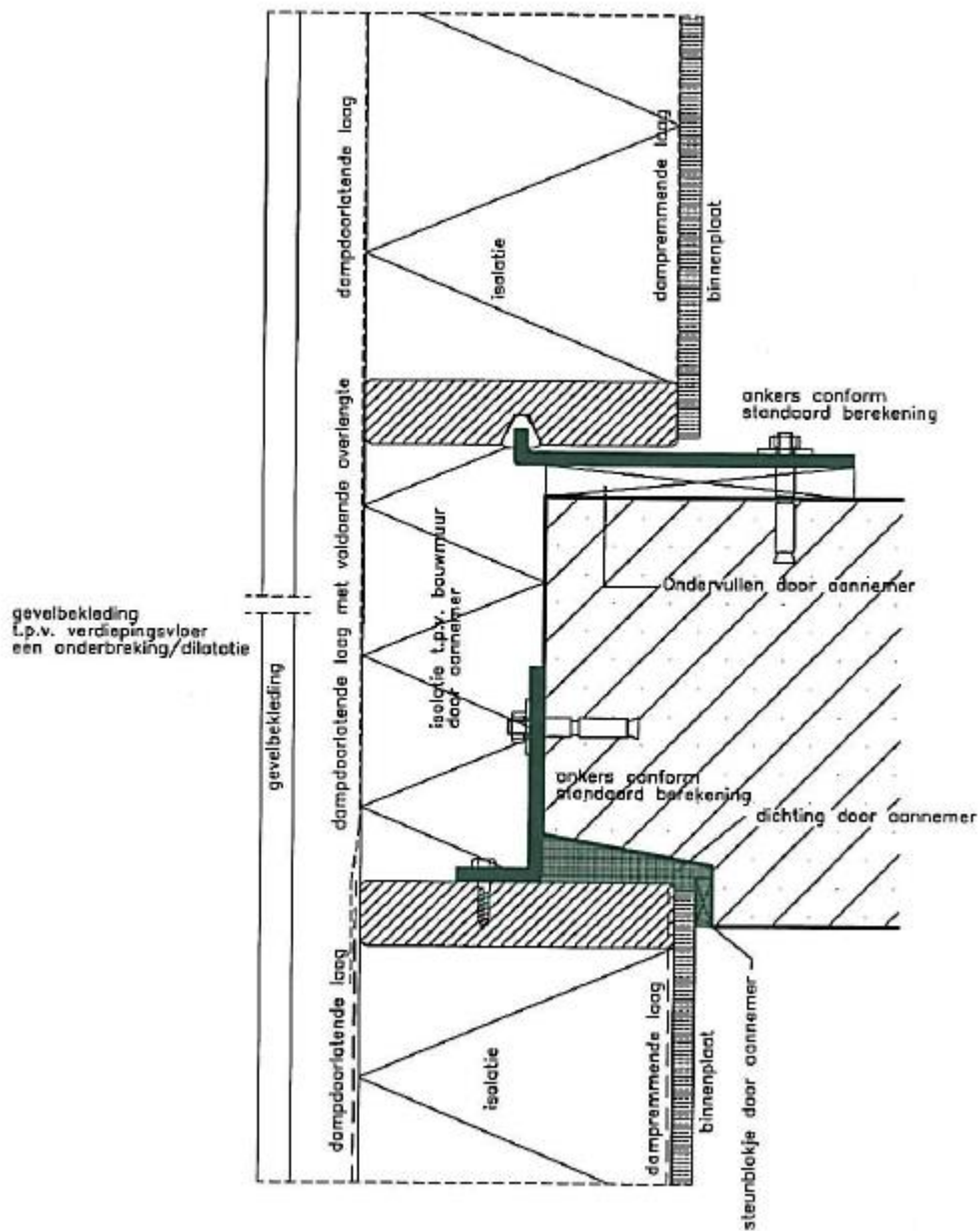
Detail 3A
