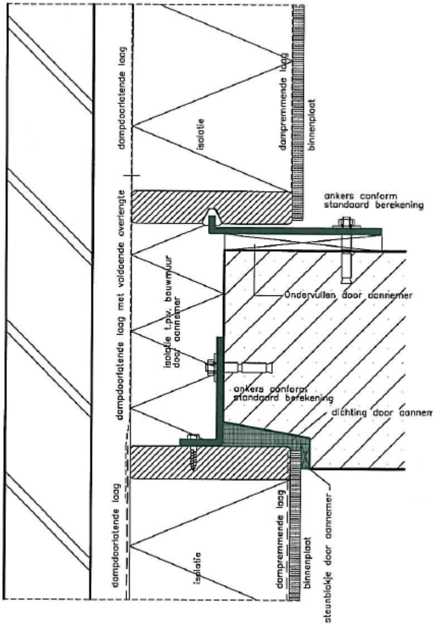
Detail 3
