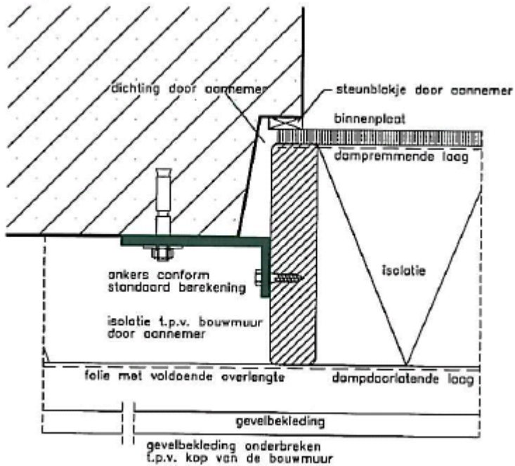
Detail 2A.
