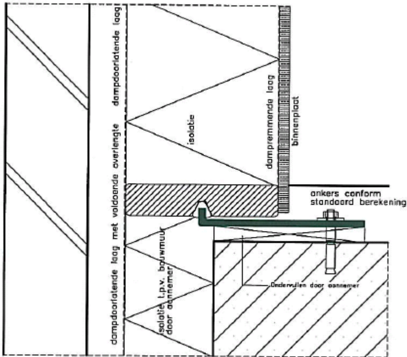
Detail 6.
