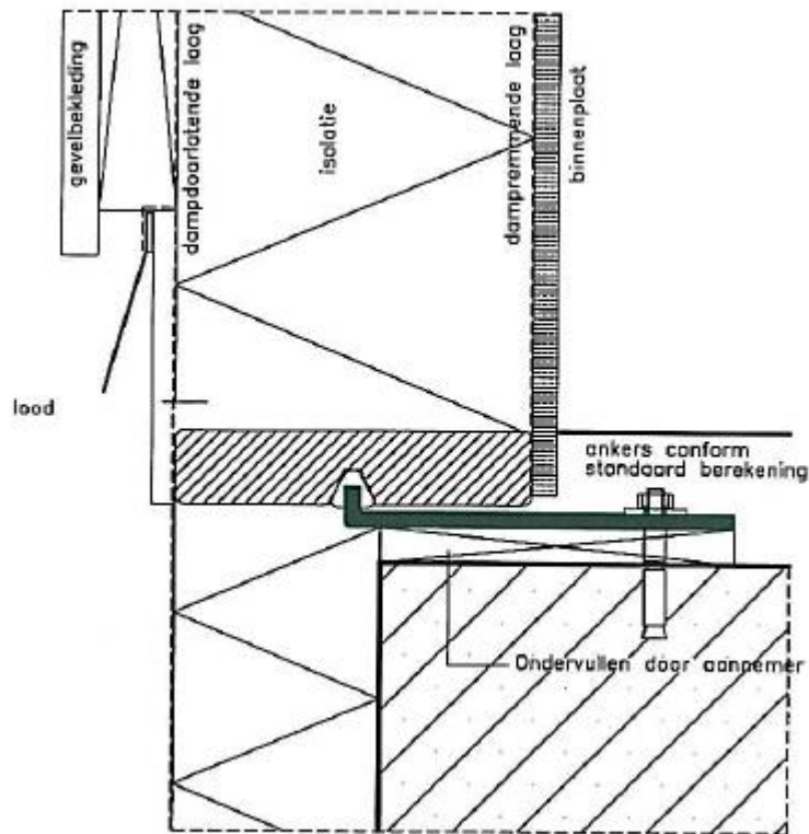
Detail 6A.
