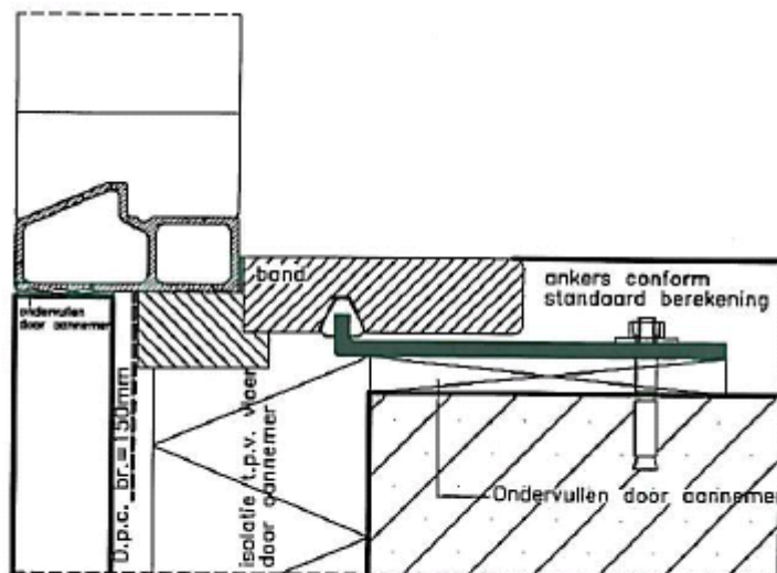
Detail 7.
