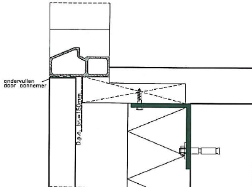
Detail 7B.
