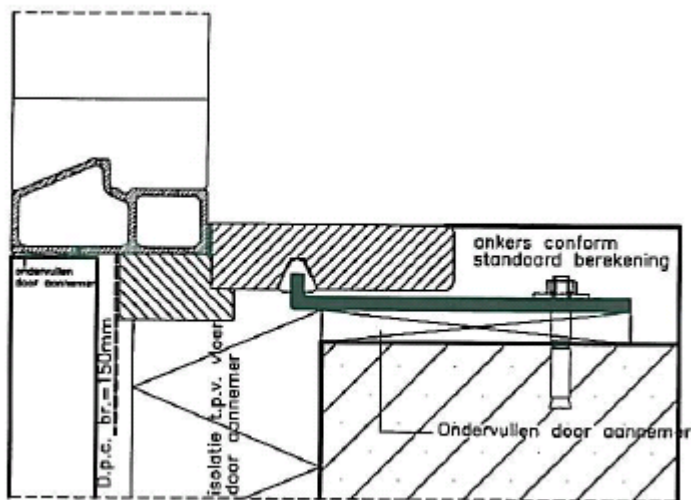
Detail 7.
