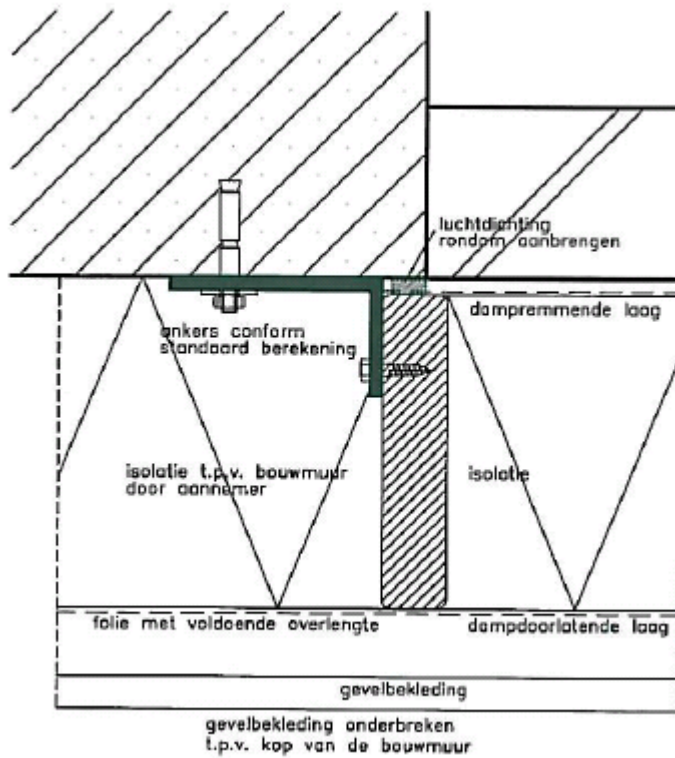
Detail 2B.
