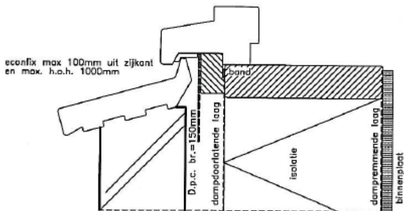
Detail 5.
