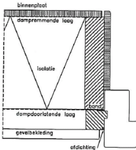
Detail 2A.
