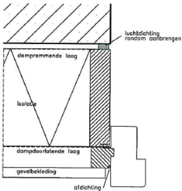
Detail 2B.
