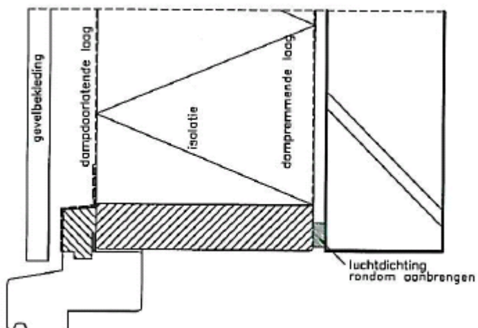
Detail 4B.
