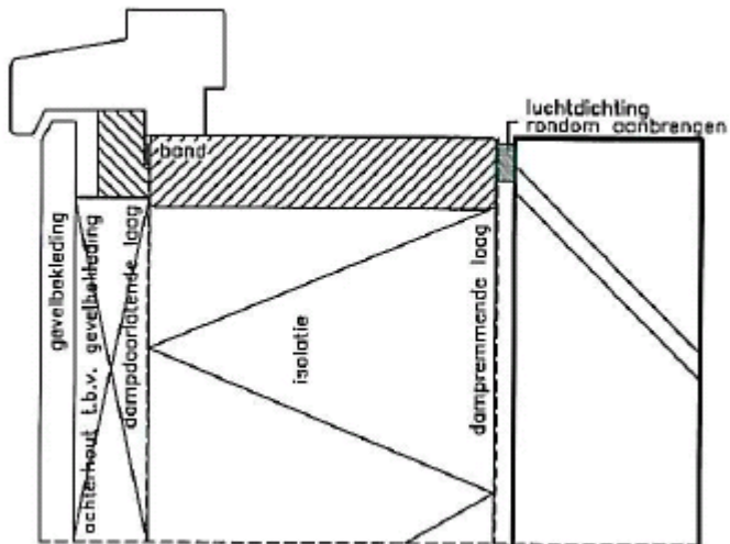
Detail 6B.
