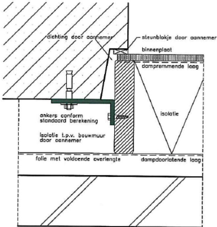
Detail 2.
