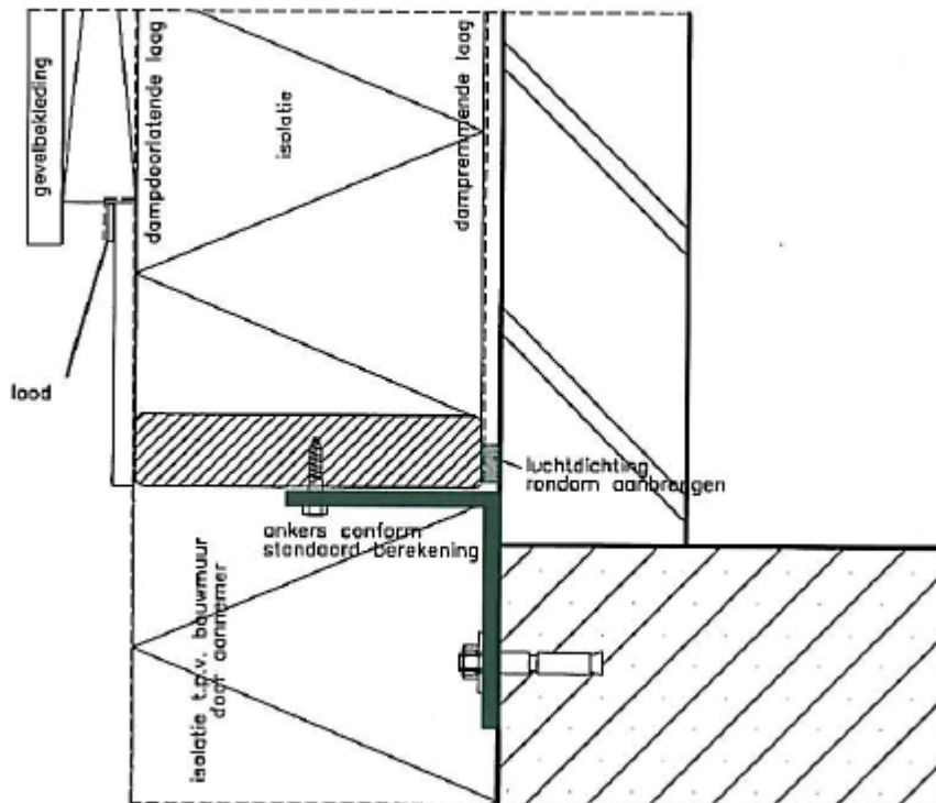
Detail 6B.
