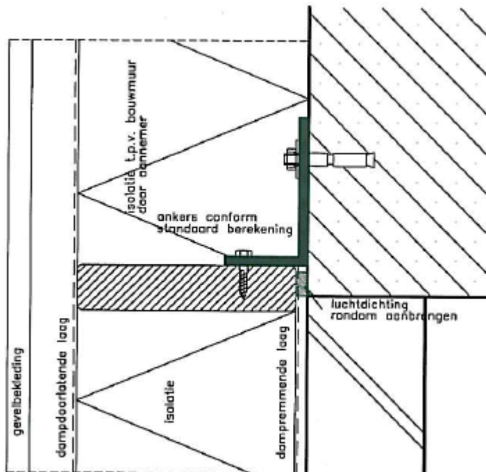
Detail 4B.
