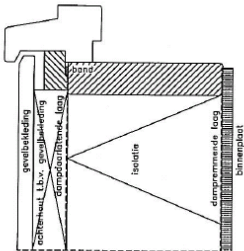
Detail 5A.
